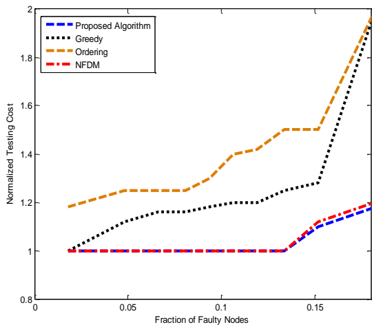
Figure (10): Normalized testing cost in scenario 2.
