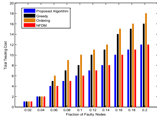
Figure (6): Total test cost in scenario 1.
